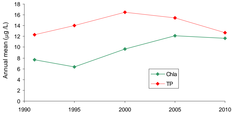
Figure 24. Correlation of annual mean total phosphorus and phytoplankton chlorophyll a concentrations. (Based on data from Lakes Tours 1991 to 2010).
