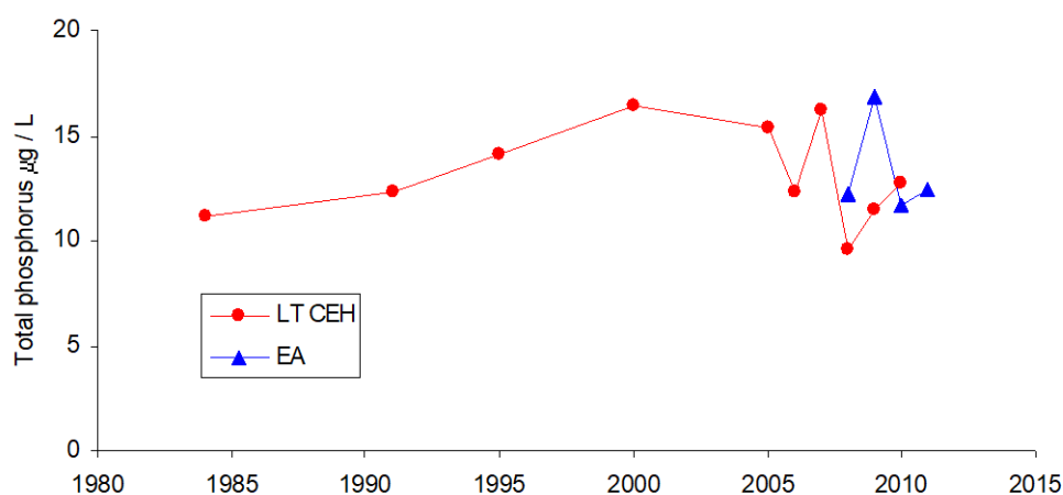
Figure 16. Annual mean concentrations of total phosphorus in Loweswater, 1984 to 2011. (From Lakes Tours, CEH and Environment Agency data).
