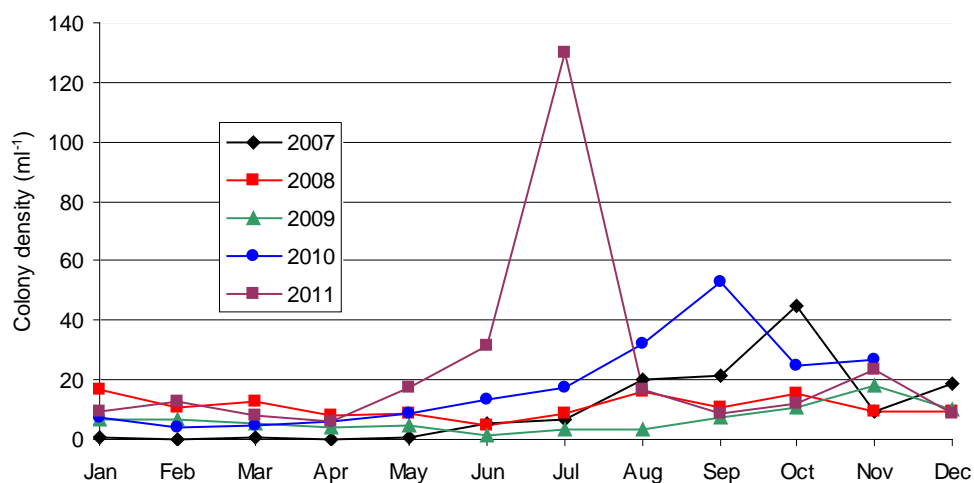
Figure 23. Seasonal variations in Woronichinia naegeliana observed in Loweswater, 2007 to 2011.
