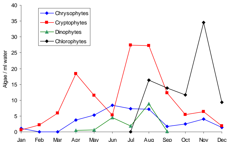
Figure 19. Seasonal variation in Chlorophyte, Chrysophyte, Cryptophyte and Dinophyte populations observed in Loweswater – 2011.
