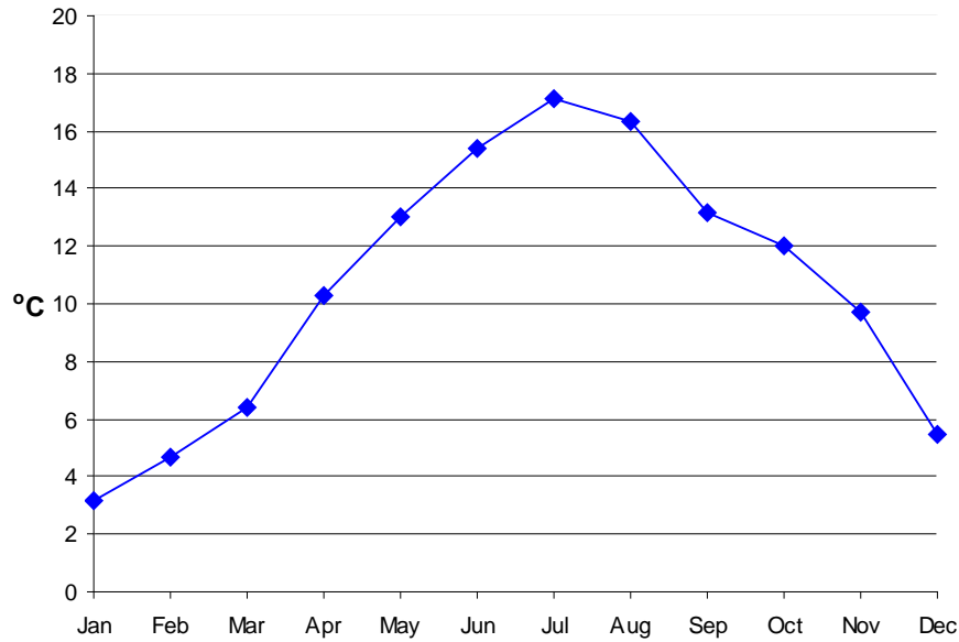
Figure 5. Seasonal variation in surface water temperature in Loweswater, 2011.
