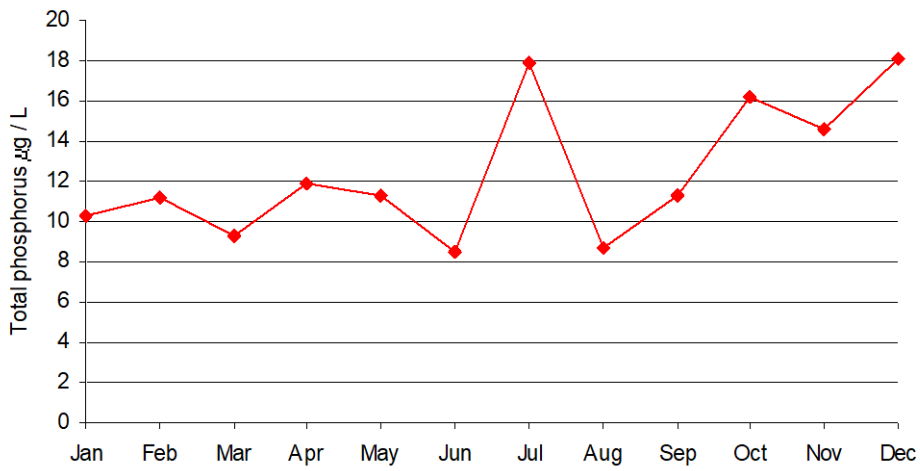
Figure 13. Seasonal variation in concentrations of total phosphorus in Loweswater, 2011.
