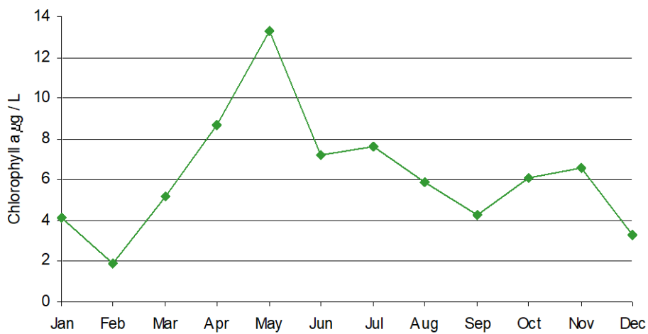
Figure 14. Seasonal variation in concentrations of phytoplankton chlorophyll a in Loweswater, 2011.
