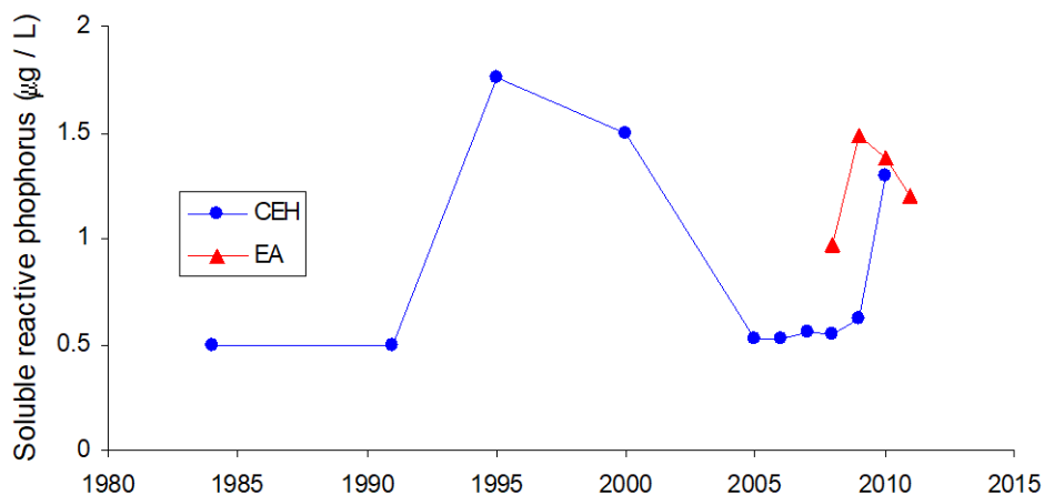
Figure 10. Annual mean concentrations of SRP in Loweswater, 1984 to 2011. (From Lakes Tours, CEH and Environment Agency data).
