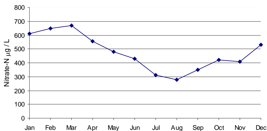
Figure 11. Seasonal variation in concentrations of nitrate-nitrogen in Loweswater, 2011.
