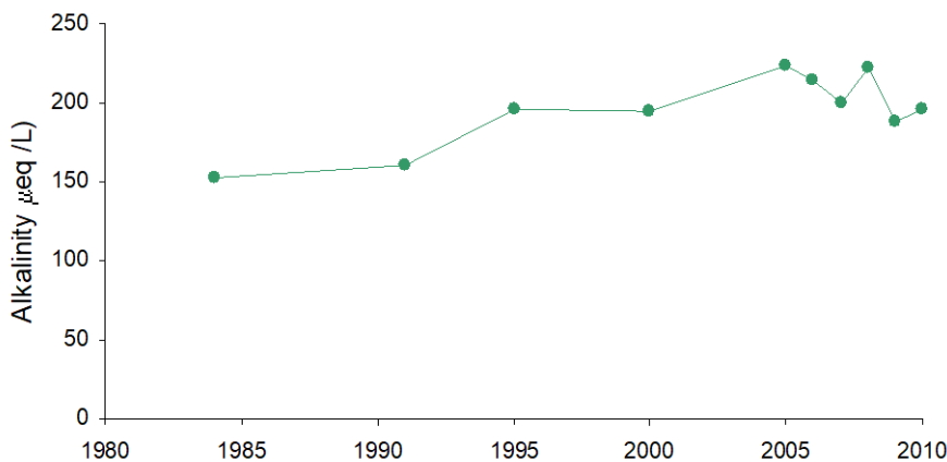
Figure 2. Annual mean values for alkalinity in Loweswater 1984 to 2010. (From Lakes Tours and CEH data)
