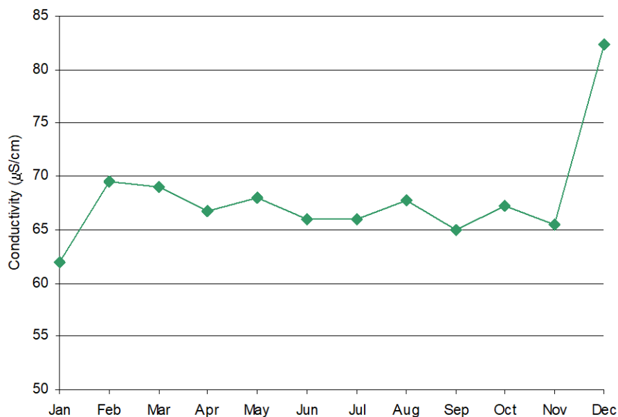
Figure 6. Seasonal changes in conductivity in Loweswater, 2011.
