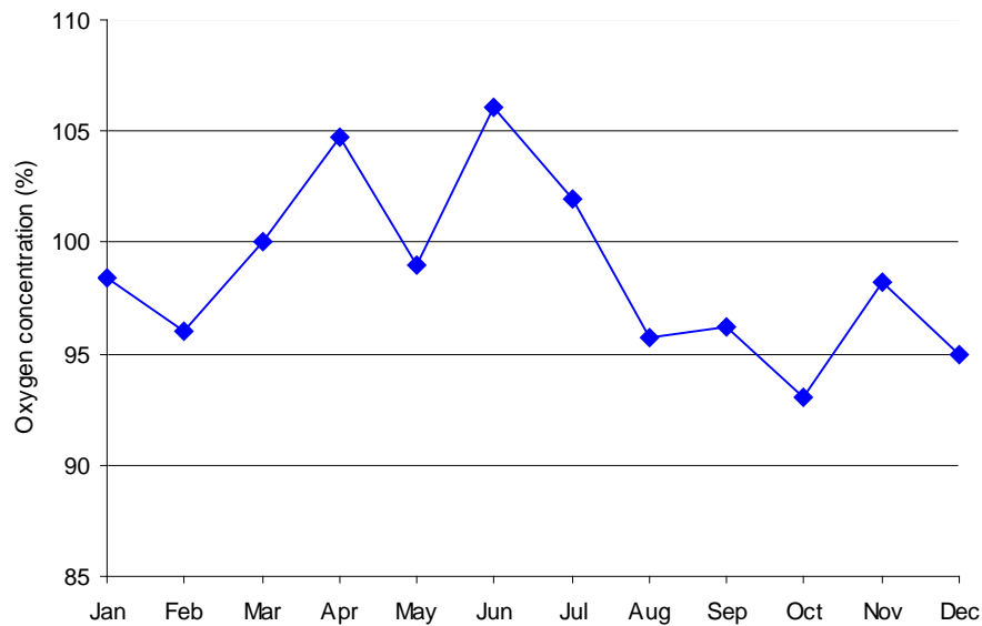
Figure 7. Seasonal variation in surface oxygen concentrations (%) in Loweswater, 2011.
