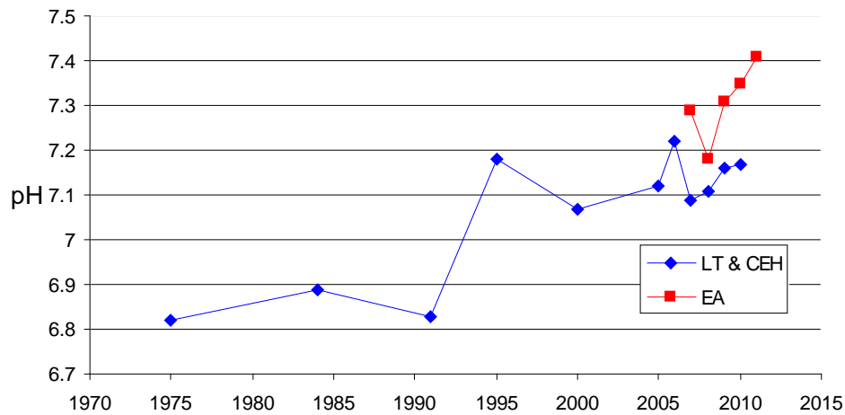
Figure 4. Annual mean pH values in Loweswater 1975 to 2011. (From Carrick and Sutcliffe, 1982; Lakes Tours, CEH and Environment Agency).
