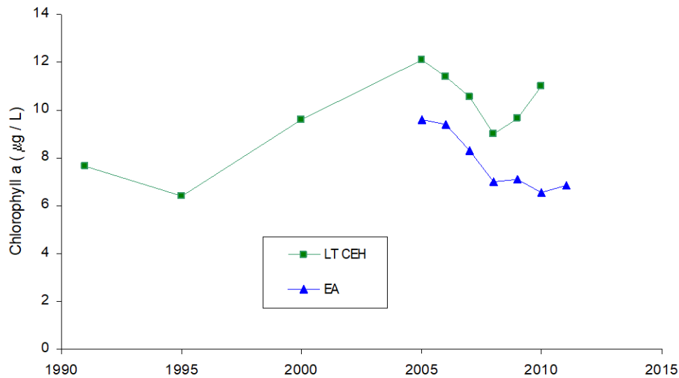
Figure 17. Annual mean concentrations of phytoplankton chlorophyll a in Loweswater, 1990 to 2011 (From Lakes Tours, CEH and Environment Agency data).
