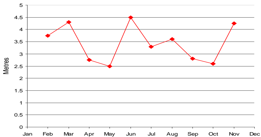
Figure 15. Seasonal changes in depth of Secchi disc in Loweswater, 2011.
