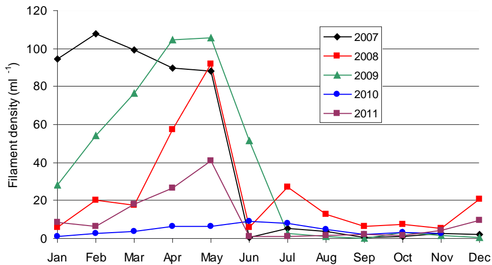
Figure 22. Seasonal variations in Planktothrix mougeotti observed in Loweswater, 2007 to 2011.
