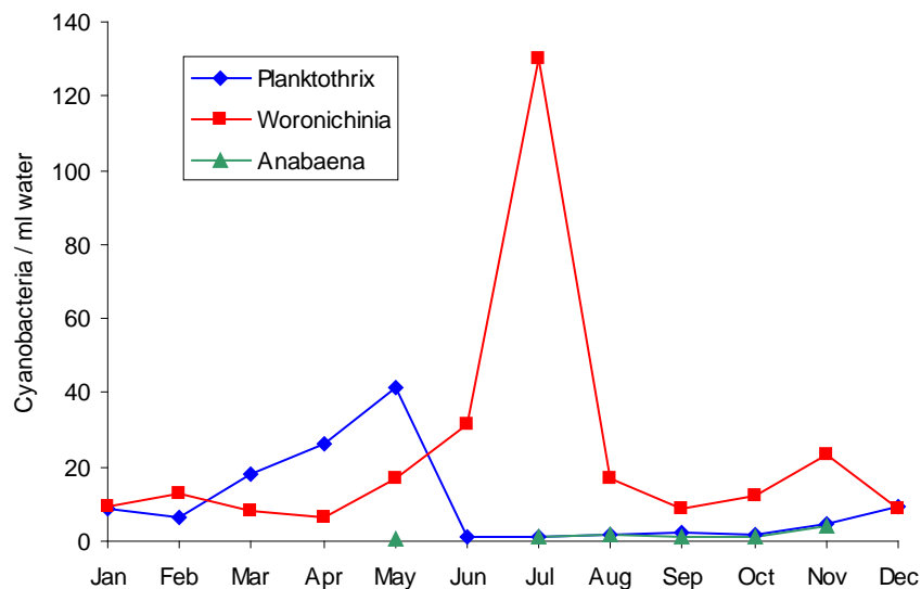
Figure 21. Seasonal variations in cyanobacterial populations observed in Loweswater - 2011
