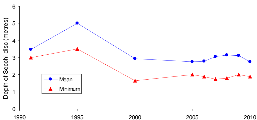
Figure 18. Annual mean and annual minimum depth of Secchi disc in Loweswater, 1991 to 2010. (CEH data).
