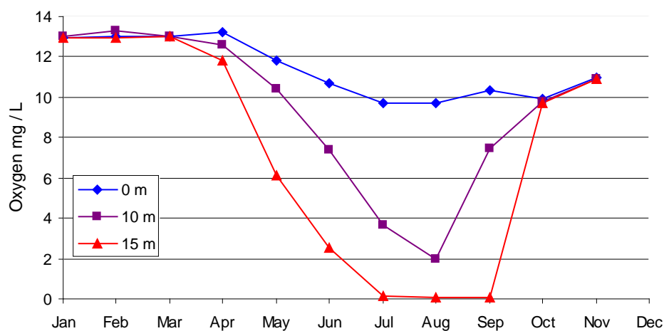
Figure 8. Seasonal variation in oxygen levels (mg / L) at 0, 10 and 15 metres in Loweswater, 2010. (from Lakes Tours data, 2010).
