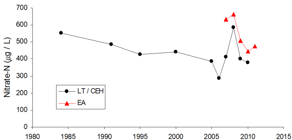
Figure 12. Annual mean concentrations of nitrate-nitrogen in Loweswater, 1984 to 2011. (From Lakes Tours, CEH and Environment Agency data ).
