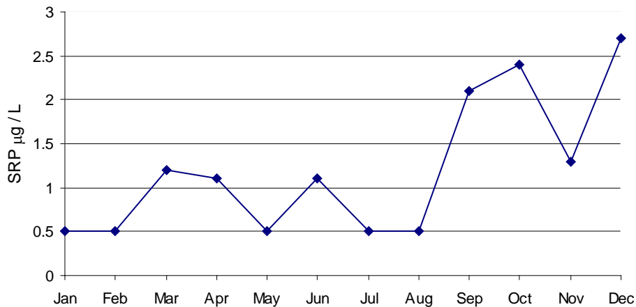
Figure 9. Seasonal variation in concentrations of SRP in Loweswater, 2011.
