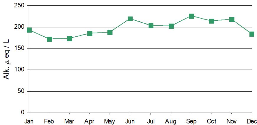
Figure 1. Seasonal changes in Alkalinity in Loweswater, 2011.
