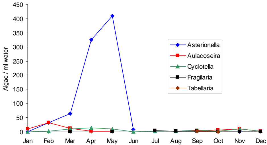
Figure 20. Seasonal variation in diatom populations observed in Loweswater – 2011.
