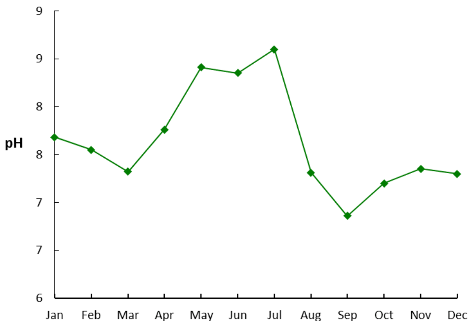
Figure 3. Seasonal variation in pH values in Loweswater, 2011.
